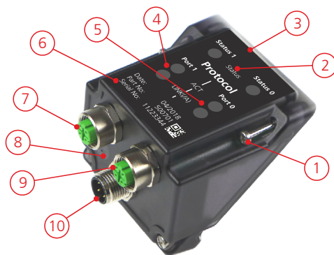
Figure 2: Components with detail information of the exchangeable cover with Industrial Ethernet
