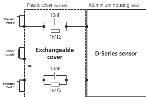
Figure 7: Shielding concept of the D-Series sensor and the exchangeable cover with Industrial Ethernet
