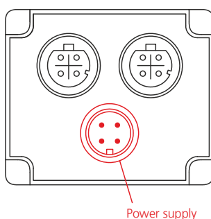
Figure 4: Connection diagram of the sensor power supply
