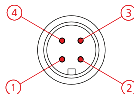
Figure 4: Connection diagram of the sensor power supply
